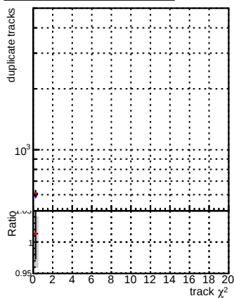
Legend: - Blue line: DQM_CKF_XiMinusNOPU_base - Red line: DQM_CKF_XiMinusNOPU_retrainOldFiles125_v2_prelimWPM_epoch3 - Gray shaded area: 1-sigma uncertainty band - Red dot: Data point - Black error bars: 1-sigma uncertainty band
