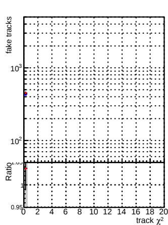
Legend: - Blue line: DQM_CKF_XiMinusNOPU_base - Red line: DQM_CKF_XiMinusNOPU_retrainOldFiles125_v2_prelimWPM_epoch3 - Gray shaded area: 1-sigma uncertainty band - Red dot: Data point - Black error bars: 1-sigma uncertainty band
