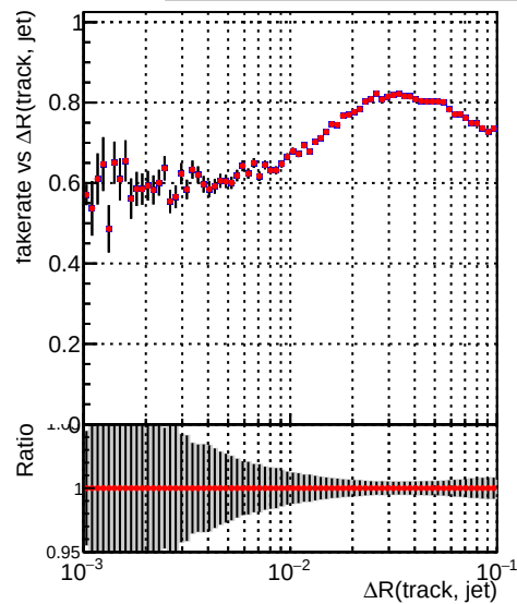
Fake rate vs \Delta R (track, jet) Legend: - ■ DQM_CKF_XiMinusNOPU_base - ■ DQM_CKF_XiMinusNOPU_retrainOldFiles125_v2_prelimWPM_epoch3
