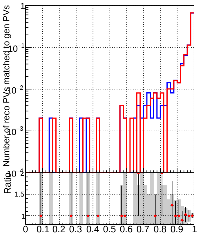
RecoPVAssoc2GenPVMatched_Purity
