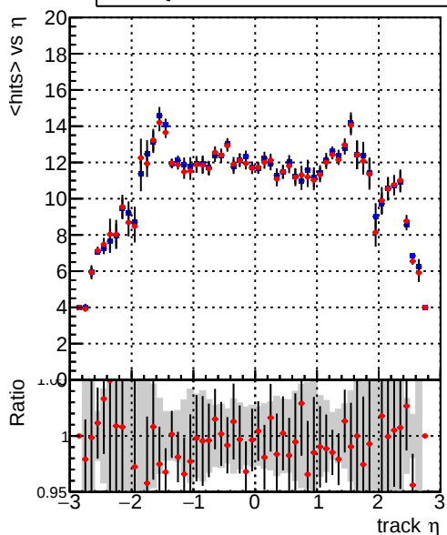
mean hits vs \eta — DQM_CKF_XiMinusNOPU_base — DQM_CKF_XiMinusNOPU_retrainOldFiles125_v2_prelimWPM_epoch3
