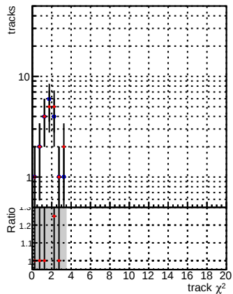
N of reco track vs. \chi^2 for DQM_CKF_XiMinusNOPU_base and DQM_CKF_XiMinusNOPU_retrainOldFiles125_v2_prelimWPM_epoch3
