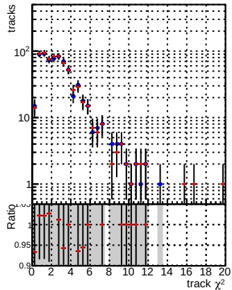
N of reco track vs. \chi^2 — DQM_CKF_XiMinusNOPU_base — DQM_CKF_XiMinusNOPU_retrainOldFiles125_v2_prelimWPM_epoch3
