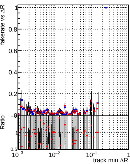
Legend: —•— DQM_CKF_XiMinusNOPU_base —•— DQM_CKF_XiMinusNOPU_retrainOldFiles125_v2_prelimWPM_epoch3
