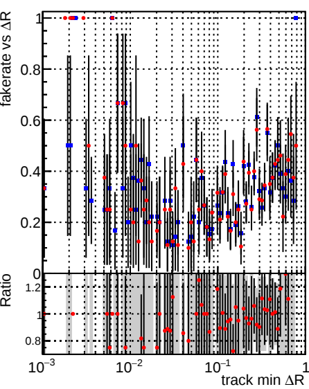
Fake rate vs \Delta R (track, jet) DQM_CKF_XiMinusNOPU_base DQM_CKF_XiMinusNOPU_retrainOldFiles125_v2_prelimWPM_epoch3
