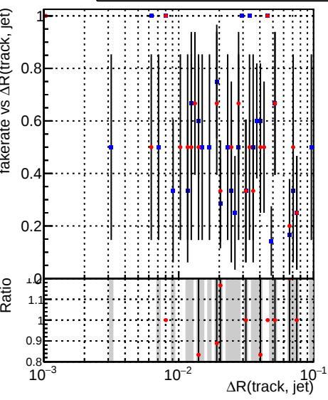
Fake rate vs \Delta R (track, jet) DQM_CKF_XiMinusNOPU_base DQM_CKF_XiMinusNOPU_retrainOldFiles125_v2_prelimWPM_epoch3
