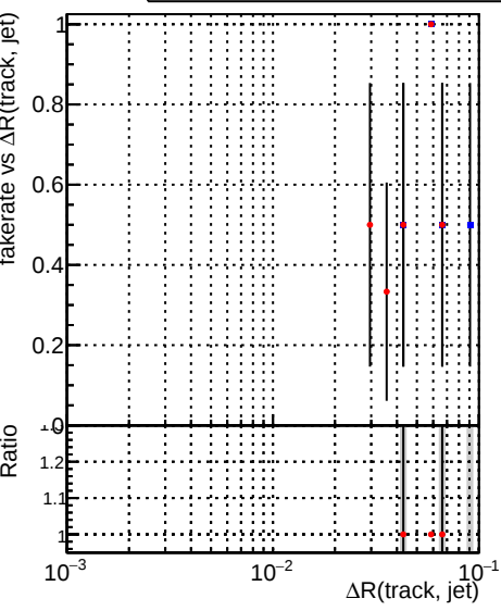
Fake rate vs \Delta R(\text{track, jet}) Legend: \blacksquare DQM_CKF_XiMinusNOPU_base \bullet DQM_CKF_XiMinusNOPU_retrainOldFiles125_v2_prelimWPM_epoch3
