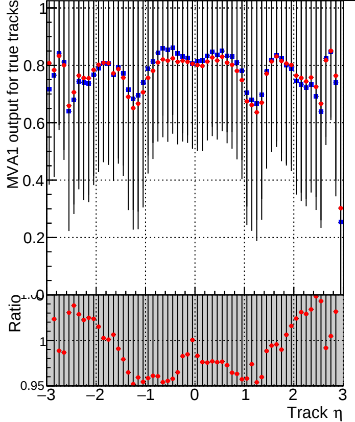
MVA1 of associated tracks (recoToSim) vs. track \eta Legend: ■ DQM_CKF_XiMinusNOPU_base ● DQM_CKF_XiMinusNOPU_retrainOldFiles125_v2_prelimWPM_epoch3
