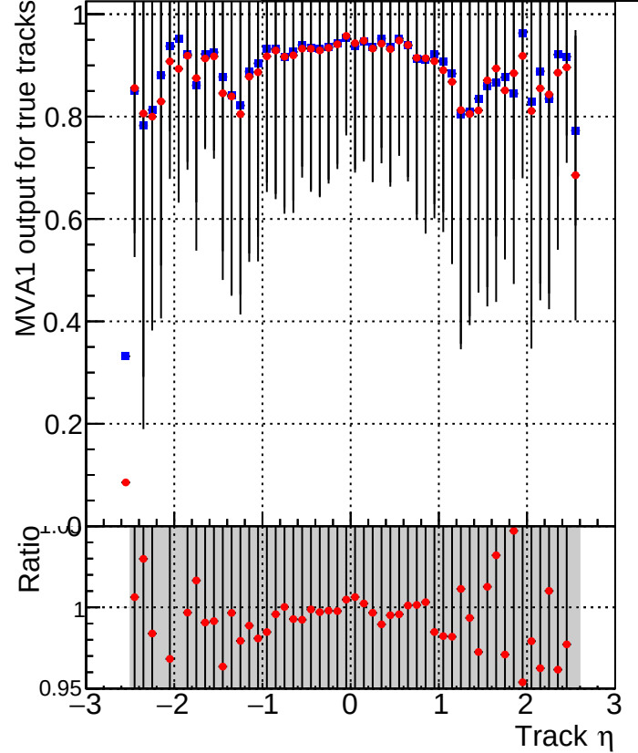
MVA1 of associated tracks (recoToSim) vs. track \eta Legend: Blue square: DQM_CKF_XiMinusNOPU_base Red diamond: DQM_CKF_XiMinusNOPU_retrainOldFiles125_v2_prelimWPM_epoch3
