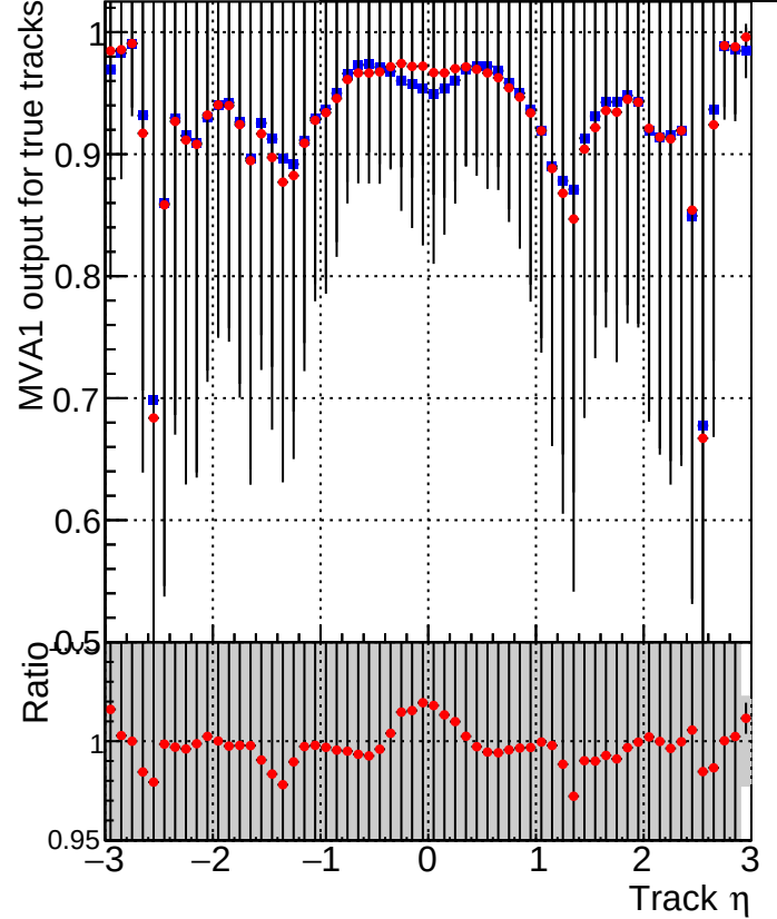
MVA1 of associated tracks (recoToSim) vs. track \eta Legend: Blue star: DQM_CKF_XiMinusNOPU_base Red diamond: DQM_CKF_XiMinusNOPU_retrainOldFiles125_v2_prelimWPM_epoch3
