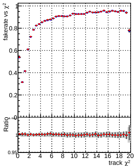
Fake rate vs. \chi^2 Legend: \square DQM_CKF_XiMinusNOPU_base \square DQM_CKF_XiMinusNOPU_retrainOldFiles125_v2_prelimWPM_epoch3
