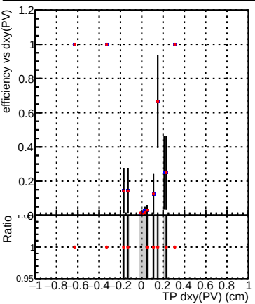
Efficiency vs Dxy(PV) plot comparing DQM_CKF_XiMinusNOPU_base (blue dots) and DQM_CKF_XiMinusNOPU_retrainOldFiles125_v2_prelimWPM_epoch3 (red line).
