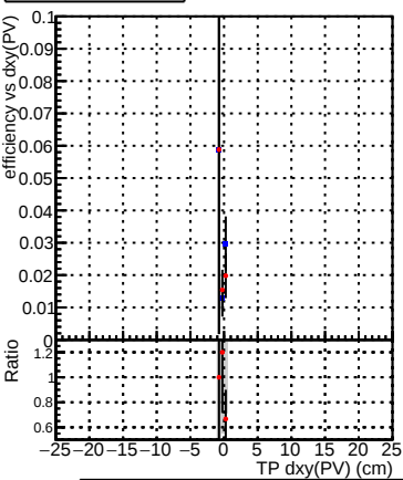
Efficiency vs Dxy(PV) plot comparing DQM_CKF_XiMinusNOPU_base (blue dots) and DQM_CKF_XiMinusNOPU_retrainOldFiles125_v2_prelimWPM_epoch3 (red line).
