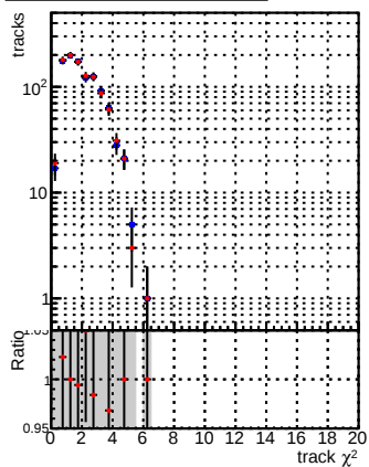
N of reco track vs. \chi^2 DQM_CKF_XiMinusNOPU_base DQM_CKF_XiMinusNOPU_retrainOldFiles125_v2_prelimWPM_epoch3
