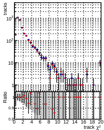
N of reco track vs. \chi^2 —●— DOM CKF XiMinusNOPU_base —●— DOM CKF XiMinusNOPU_retrainOldFiles125_v2_prelimWPM_epoch3
