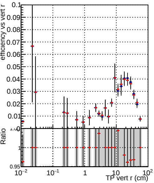
Efficiency vs vertpos Legend: DQM_CKF_XiMinusNOPU_base DQM_CKF_XiMinusNOPU_retrainOldFiles125_v2_prelimWPM_epoch2
