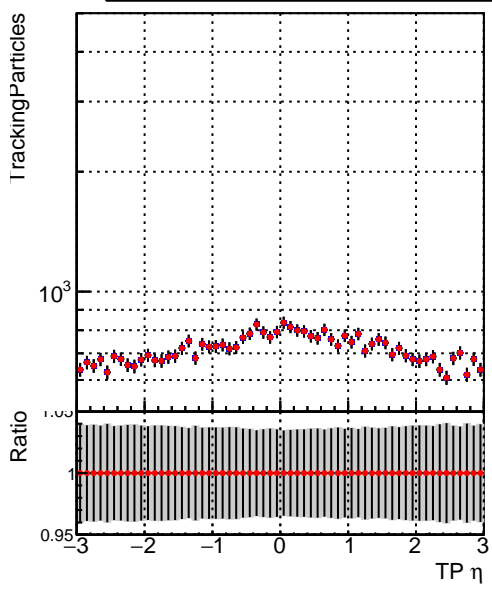
N of simulated tracks vs TP \eta Legend: — DQM_CKF_XiMinusNOPU_base — DQM_CKF_XiMinusNOPU_retrainOldFiles125_v2_prelimWPM_epoch2
