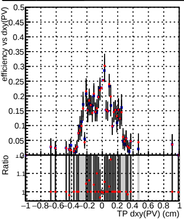
Efficiency vs Dxy(PV) plot comparing DQM_CKF_XiMinusNOPU_base (black squares) and DQM_CKF_XiMinusNOPU_retrainOldFiles125_v2_prelimWPM_epoch2 (red circles).
