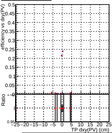
Efficiency vs Dxy(PV) plot comparing DQM_CKF_XiMinusNOPU_base (black squares) and DQM_CKF_XiMinusNOPU_retrainOldFiles125_v2_prelimWPM_epoch2 (red circles).
