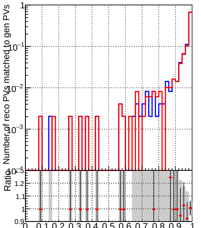
RecoPVAssoc2GenPVMatched_Purity
