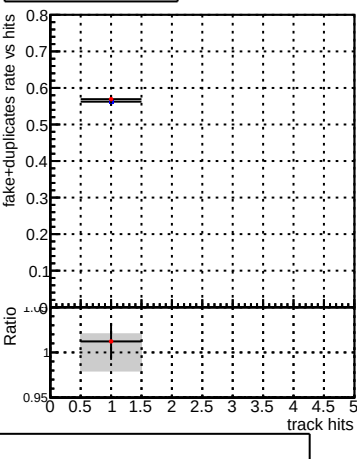
fake+duplicates
