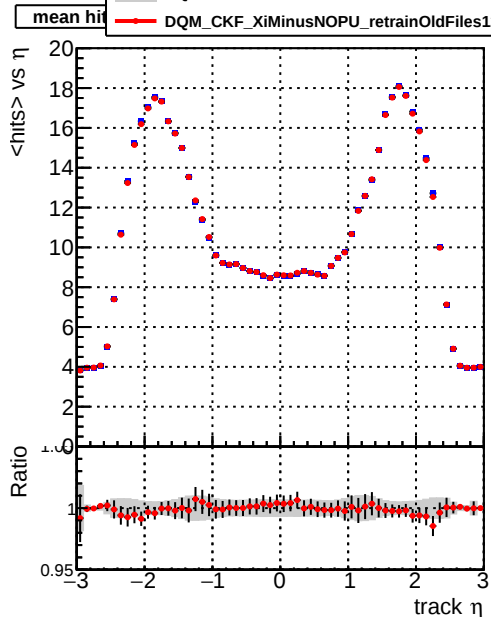
mean hits > \eta
