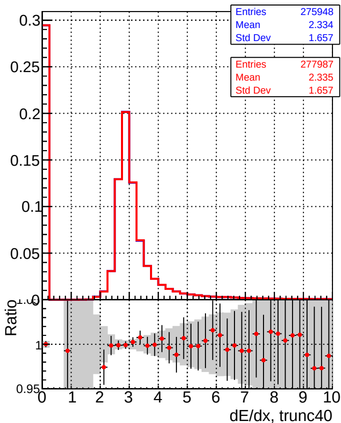
Legend: DQM_CKF_XiMinusNOPU_base (grey shaded area) DQM_CKF_XiMinusNOPU_retrainOldFiles125_v2_prelimWPM_epoch2 (red line with points)
