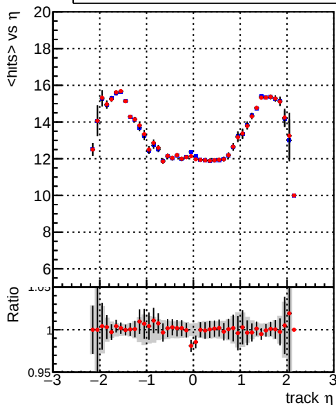
mean hit — DQM_CKF_XiMinusNOPU_base — DQM_CKF_XiMinusNOPU_retrainOldFiles125_v2_prelimWPM_epoch2
