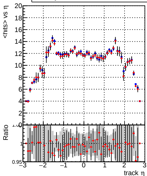
mean hits vs \eta — DQM_CKF_XiMinusNOPU_base — DQM_CKF_XiMinusNOPU_retrainOldFiles125_v2_prelimWPM_epoch2
