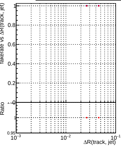
Legend: DQM_CKF_XiMinusNOPU_base (blue dots), DQM_CKF_XiMinusNOPU_retrainOldFiles125_v2_prelimWPM_epoch2 (red dots)
