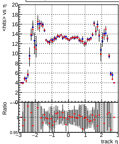
mean hits vs \eta Legend: DQM_CKF_XiMinusNOPU_base (blue line), DQM_CKF_XiMinusNOPU_retrainOldFiles125_v2_prelimWPM_epoch2 (red line)
