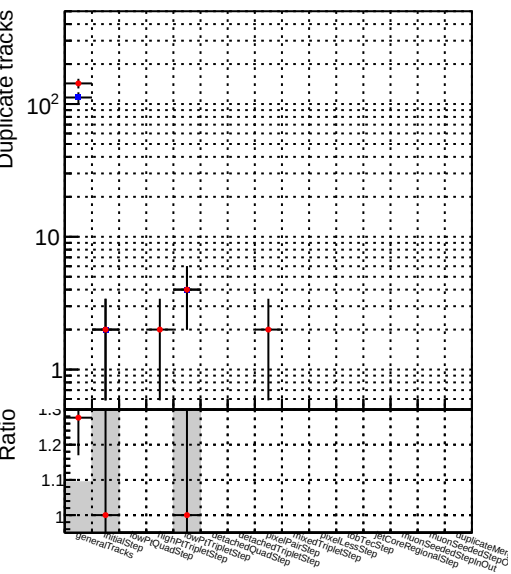
Number 1 DQM_CKF_XiMinusNOPU_retrainOldFiles125_v2_prelimWPM_epoch2
