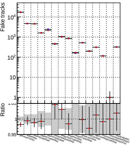
Number 1 DQM_CKF_XiMinusNOPU_retrainOldFiles125_v2_prelimWPM_epoch2
