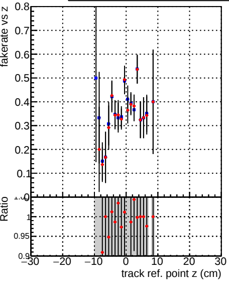
Legend: DQM_CKF_XiMinusNOPU_base (blue diamonds), DQM_CKF_XiMinusNOPU_retrainOldFiles125_v2_prelimWPM_epoch2 (red circles)
