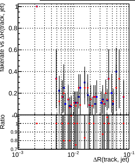
Legend: DQM_CKF_XiMinusNOPU_base (blue diamonds), DQM_CKF_XiMinusNOPU_retrainOldFiles125_v2_prelimWPM_epoch2 (red diamonds)
