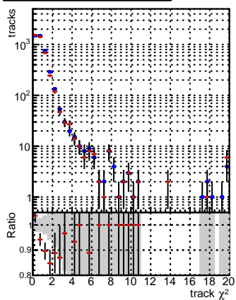
N of reco track vs. \chi^2 for DQM_CKF_XiMinusNOPU_base and DQM_CKF_XiMinusNOPU_retrainOldFiles125_v2_prelimWPM_epoch2 models.
