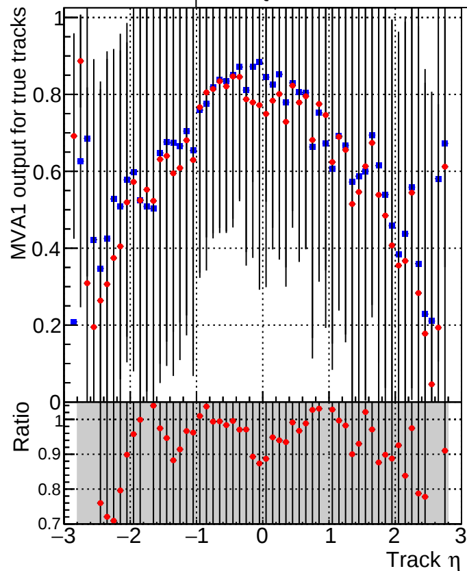
MVA1 of associated tracks (recoToSim) vs. track \eta Legend: ■ DQM_CKF_XiMinusNOPU_base ● DQM_CKF_XiMinusNOPU_retrainOldFiles125_v2_prelimWPM_epoch2
