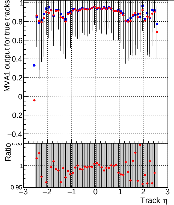
MVA1 of associated tracks (recoToSim) vs. track \eta Legend: ■ DQM_CKF_XiMinusNOPU_base ◆ DQM_CKF_XiMinusNOPU_retrainOldFiles125_v2_prelimWPM_epoch2
