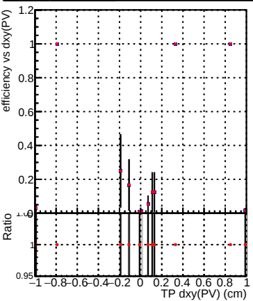
Efficiency vs Dxy(PV) (cm) - DQM_CKF_XiMinusNOPU_retrainOldFiles125_v2_prelimWPM_epoch2
