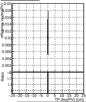
Efficiency vs Dxy(PV) - DQM_CKF_XiMinusNOPU_base (grey band) and DQM_CKF_XiMinusNOPU_retrainOldFiles125_v2_prelimWPM_epoch2 (red dots)
