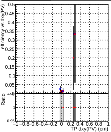
Efficiency vs Dxy(PV) - DQM_CKF_XiMinusNOPU_base (grey band) and DQM_CKF_XiMinusNOPU_retrainOldFiles125_v2_prelimWPM_epoch2 (red dots)
