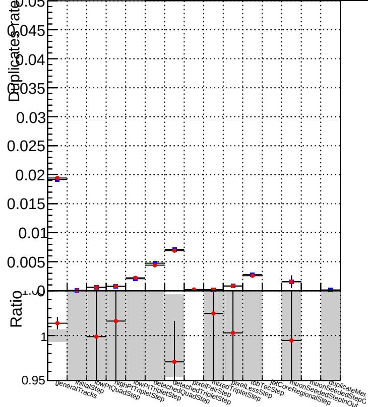
Duplicates rate vs collection Legend: DQM_CKF_XiMinusNOPU_base (Blue square) DQM_CKF_XiMinusNOPU_retrainOldFiles125_v2_prelimWPM_epoch2 (Red circle)
