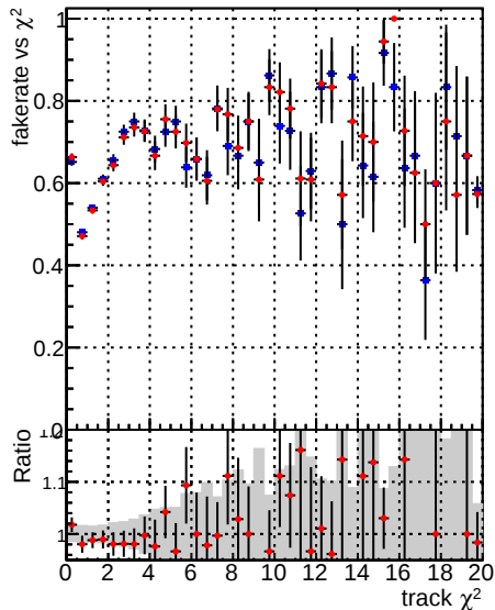
Fake rate vs. —♦— DQM_CKF_XiMinusNOPU_base —●— DQM_CKF_XiMinusNOPU_retrainOldFiles125_v2_prelimWPM_epoch2
