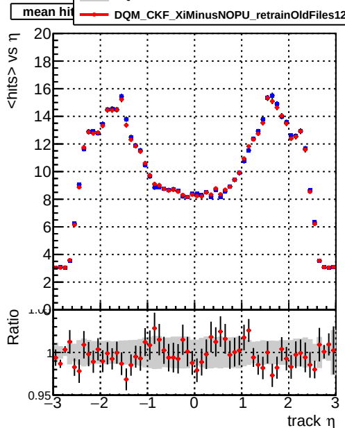
mean hits vs \eta
