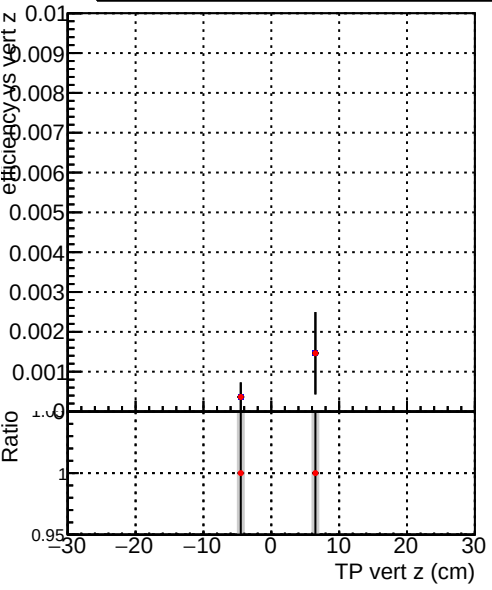
Efficiency vs vertpos Legend: DQM_CKF_XiMinusNOPU_base DQM_CKF_XiMinusNOPU_retrainOldFiles125_v2_prelimWPM_epoch1
