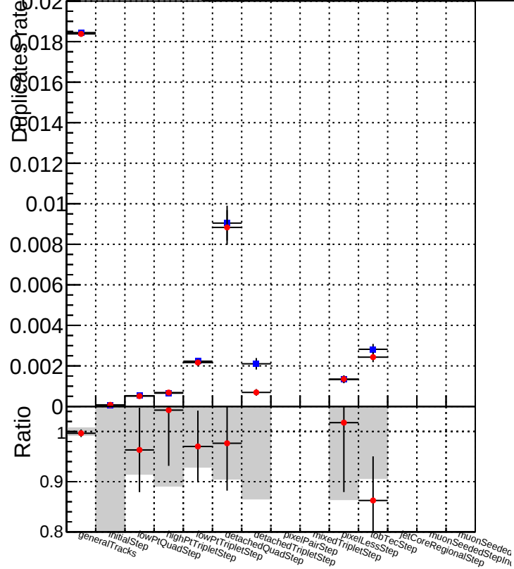
Duplicates rate vs collection Legend: DQM_CKF_XiMinusNOPU_base (blue square) DQM_CKF_XiMinusNOPU_retrainOldFiles125_v2_prelimWPM_epoch1 (red circle)
