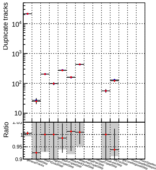
DQM_CKF_XiMinusNOPU_retrainOldFiles125_v2_prelimWPM_epoch1
