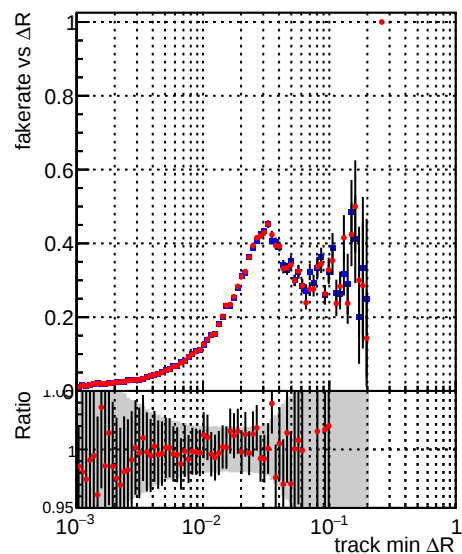
Fake rate vs \Delta R (track, jet) Legend: DQM_CKF_XiMinusNOPU_base (black line with blue markers) DQM_CKF_XiMinusNOPU_retrainOldFiles125_v2_prelimWPM_epoch1 (red line with red markers)
