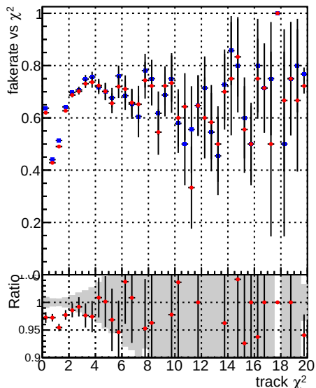
Fake rate vs. \chi^2 Legend: —•— DQM CKF XMinusNOPU_base —•— DQM CKF XMinusNOPU_retrainOldFiles125_v2_prelimWPM_epoch1
