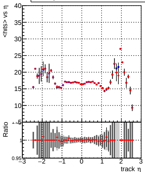
mean hits vs \eta Legend: DQM_CKF_XiMinusNOPU_base (blue line), DQM_CKF_XiMinusNOPU_retrainOldFiles125_v2_prelimWPM_epoch1 (red line)
