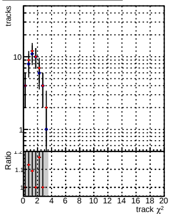
N of reco track vs. \chi^2 DQM_CKF_XiMinusNOPU_base DQM_CKF_XiMinusNOPU_retrainOldFiles125_v2_prelimWPM_epoch1
