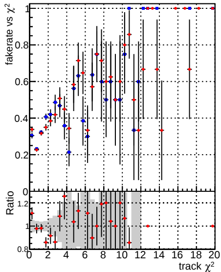
Fake rate vs. —•— DQM_CKF_XiMinusNOPU_base —•— DQM_CKF_XiMinusNOPU_retrainOldFiles125_v2_prelimWPM_epoch1
