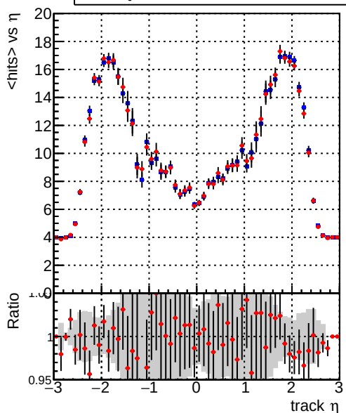
mean hits vs \eta — DQM_CKF_XiMinusNOPU_base — DQM_CKF_XiMinusNOPU_retrainOldFiles125_v2_prelimWPM_epoch1
