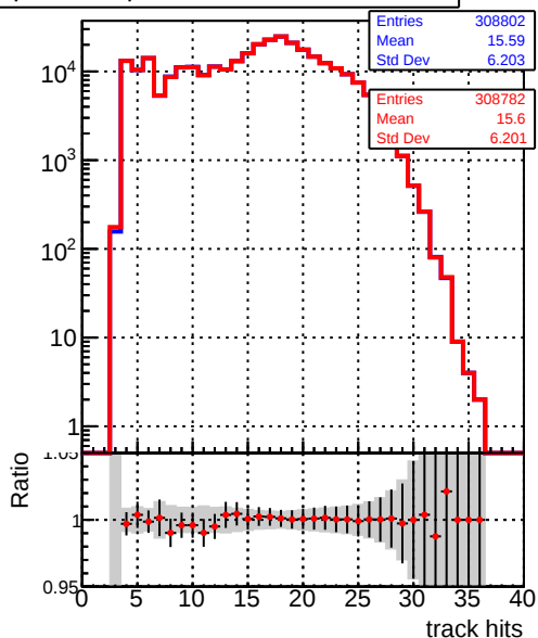
DQM_CKF_XiMinusNOPU_retrainOldFiles125_v2_prelimWPM_epoch1
