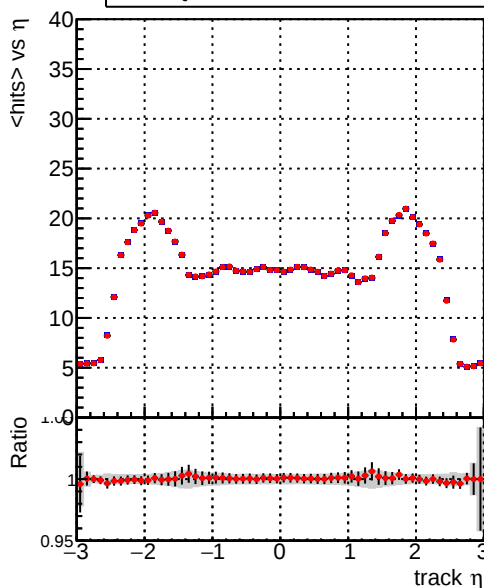
DQM_CKF_XiMinusNOPU_retrainOldFiles125_v2_prelimWPM_epoch1
