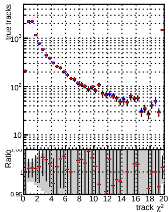
N of reco track vs. \chi^2 for DQM CKF XiMinusNOPU_base and DQM CKF XiMinusNOPU_retrainOldFiles125_v2_prelimWPM_epoch1
