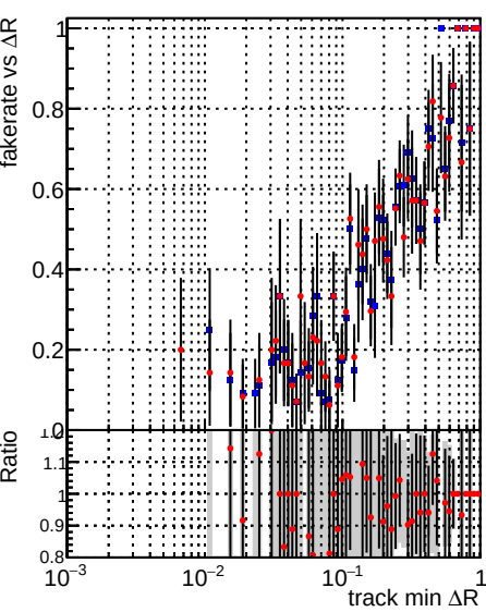
Legend: DQM_CKF_XiMinusNOPU_base (blue dots), DQM_CKF_XiMinusNOPU_retrainOldFiles125_v2_prelimWPM_epoch1 (red dots)
